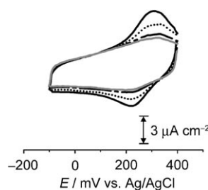
Figure 2. Cyclic voltammograms of [Cu II ( cis -L)]/C 6 -Au before (black solid line) and after irradiation with visible light for 90 min (dotted line), 180 min (hashed solid line), and 270 min (gray solid line). The SAM before light irradiation corresponds to that after 70 scans in Figure 1. The modified Au surface was irradiated with visible light in aqueous 0.1 M NaClO 4 solution. After irradiation, the electrolyte solutions were renewed before the cyclic voltammograms were measured.
