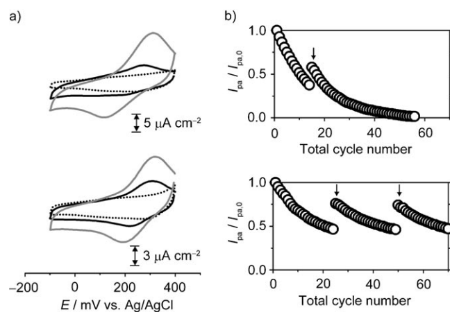
Figure 1. a) Cyclic voltammograms of L/ \text{C}_6\text{-Au} (dotted line) and [\text{Cu}^{\text{II}}(\text{L})]/\text{C}_6\text{-Au} (gray solid line, 1st scan; black solid line, 70th scan) in aqueous 0.1 M \text{NaClO}_4 solution: trans (upper) and cis forms (lower). Scan rate, 50 \text{ mV s}^{-1} . b) Plots of the relative anodic peak current ( I_{\text{pa}}/I_{\text{pa},0} ) versus the total cycle number for [\text{Cu}^{\text{II}}(\text{L})]/\text{C}_6\text{-Au} (upper, trans form; lower, cis form). The anodic peak current ( I_{\text{pa}} ) is normalized to that of the first cycle ( I_{\text{pa},0} ). The arrows in (b) represent the first scan after an interval (10–20 s) in the consecutive scans.
