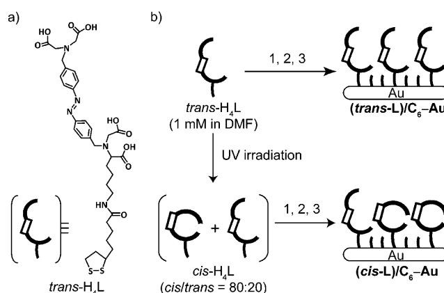
Scheme 1. a) Azobenzene ligand, trans -H 4 L. b) Preparation of the SAMs of L: 1) modification of H 4 L to an Au surface (H 4 L-Au), 2) modification of hexanethiol (C 6 ) to H 4 L-Au (H 4 L/C 6 -Au), 3) deprotonation of H 4 L/C 6 -Au (L/C 6 -Au). DMF = dimethylformamide.
